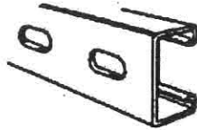
PS 520 EH CHANNEL 1-1/8" x 9/16" ELONGATED HOLES ON 2" CENTERS 1-5/8" x 13/16" x 12 GA.
